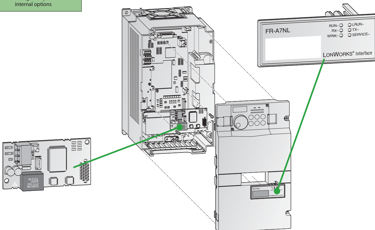
Mounting examples for internal options
